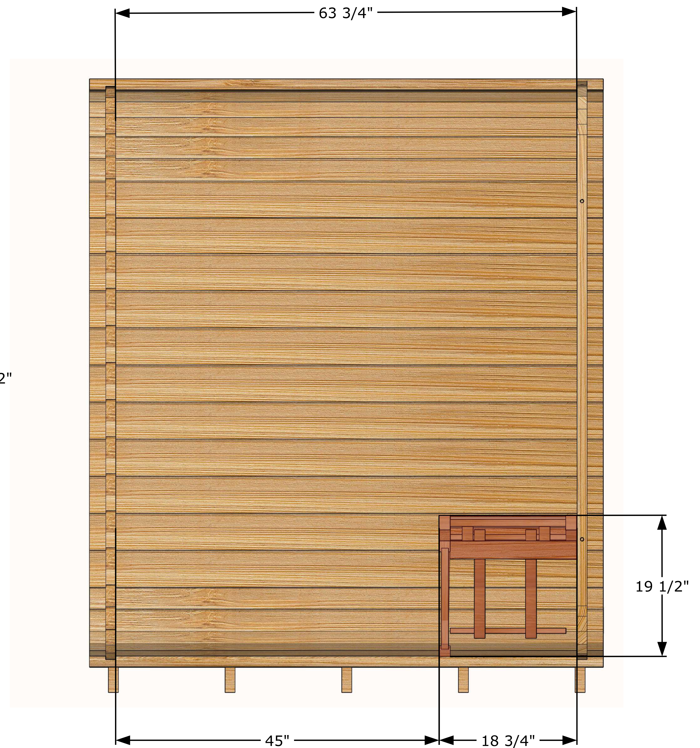
Side View
