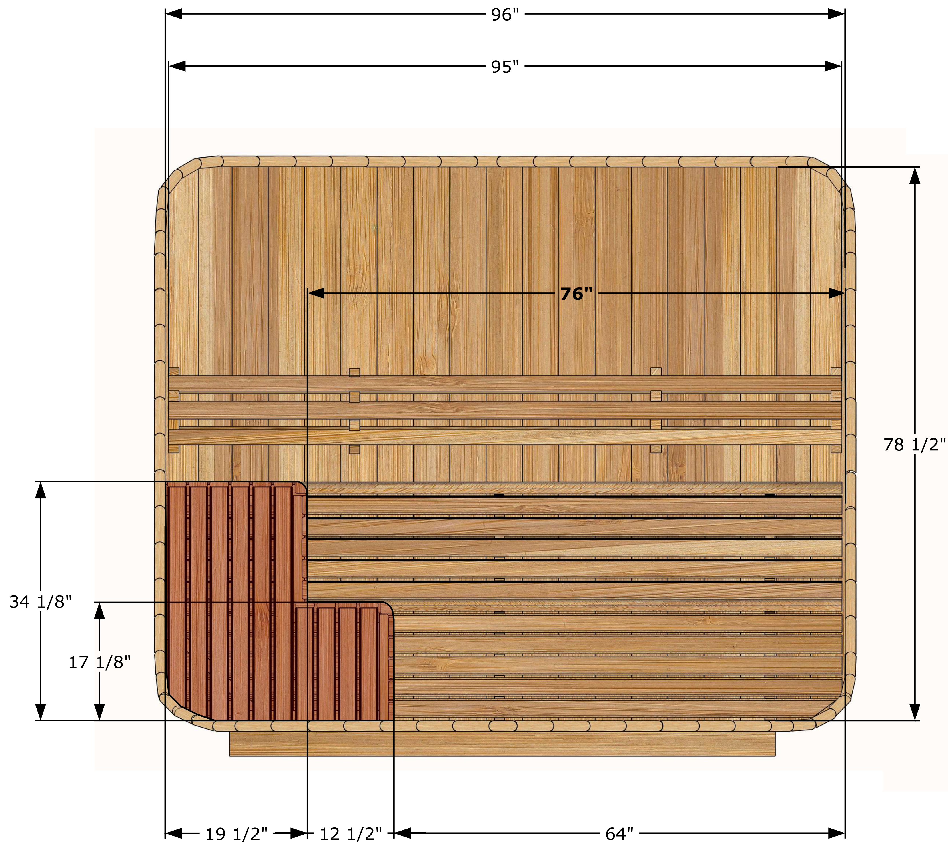
Front View
