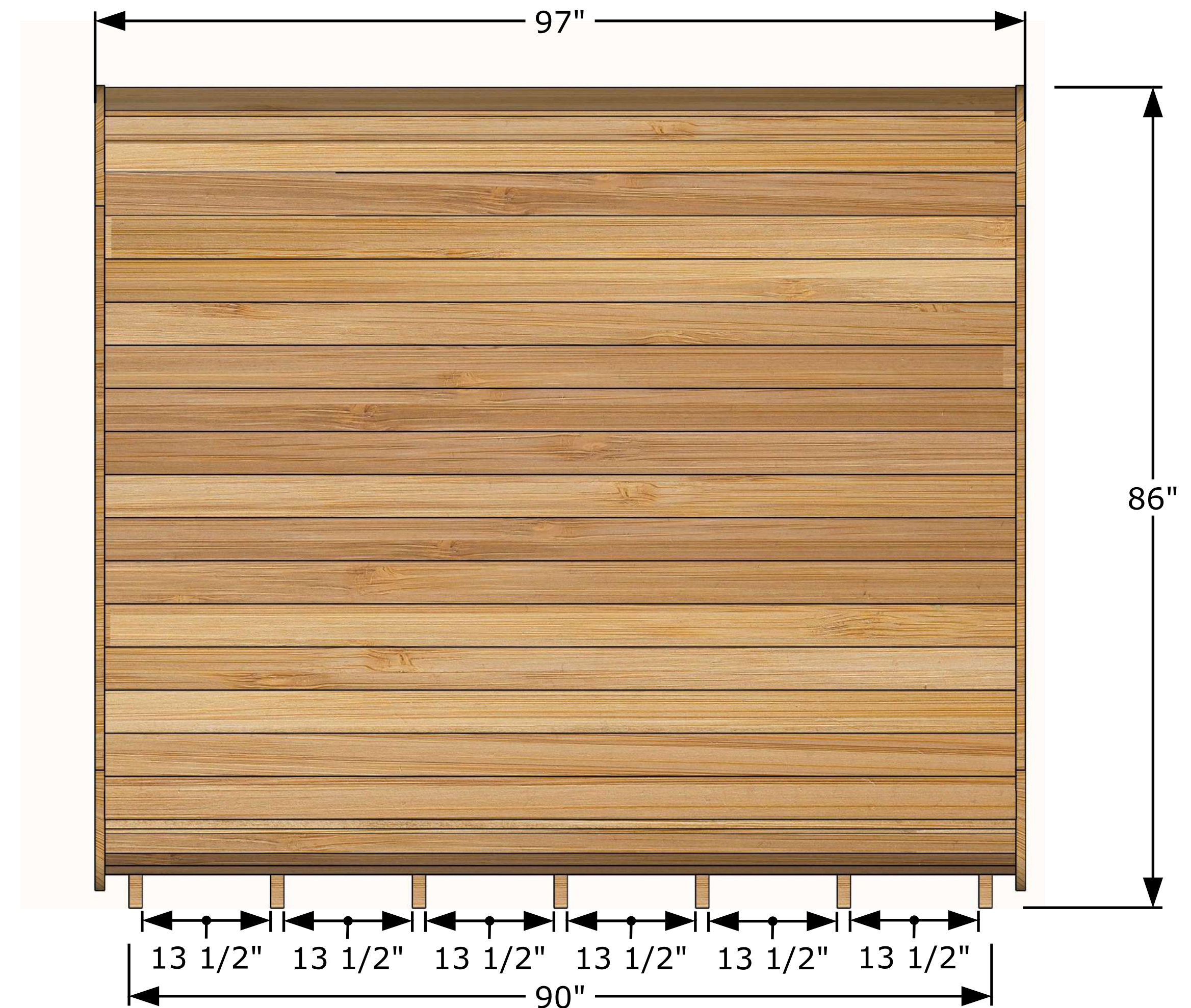
Side View
