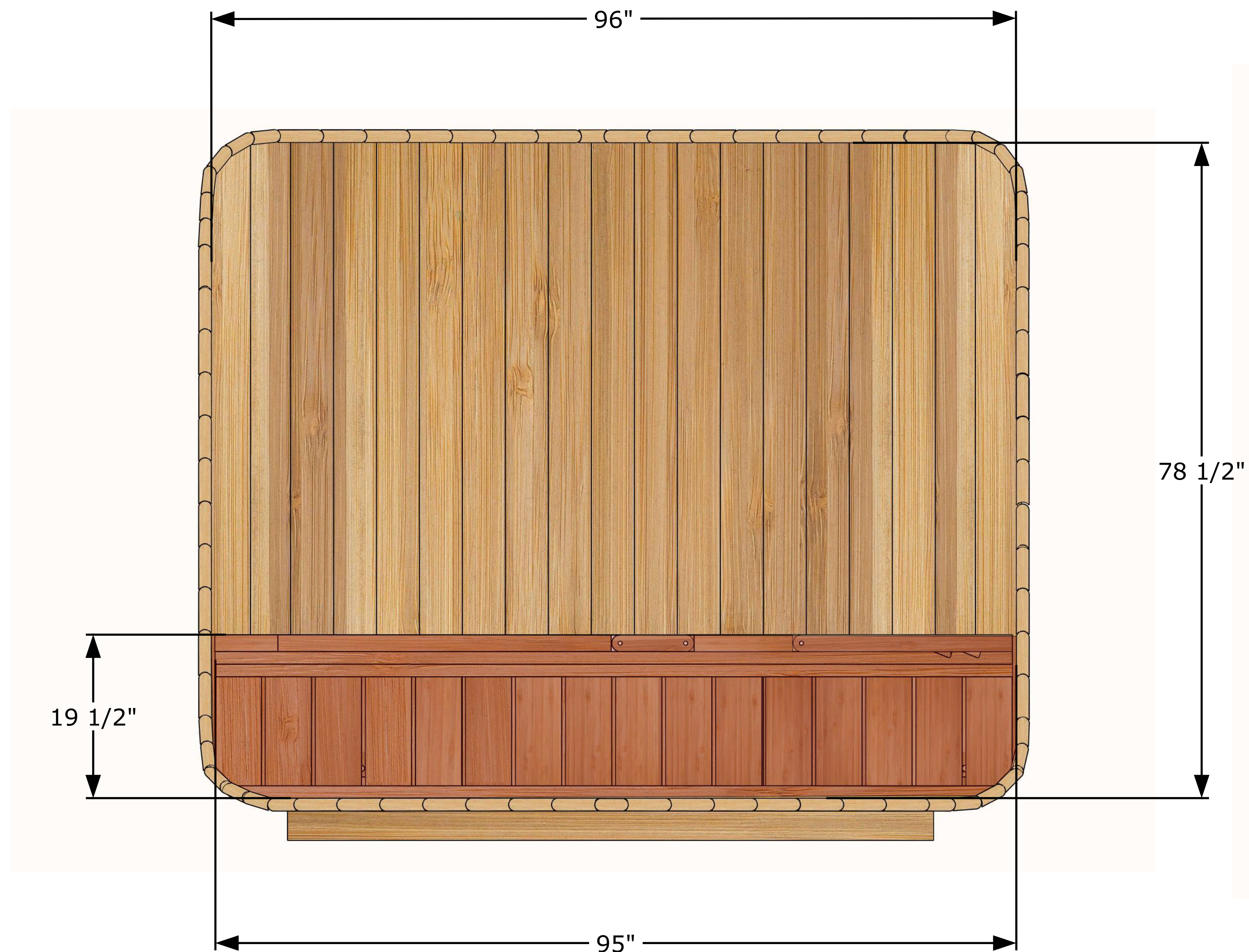
Front View
