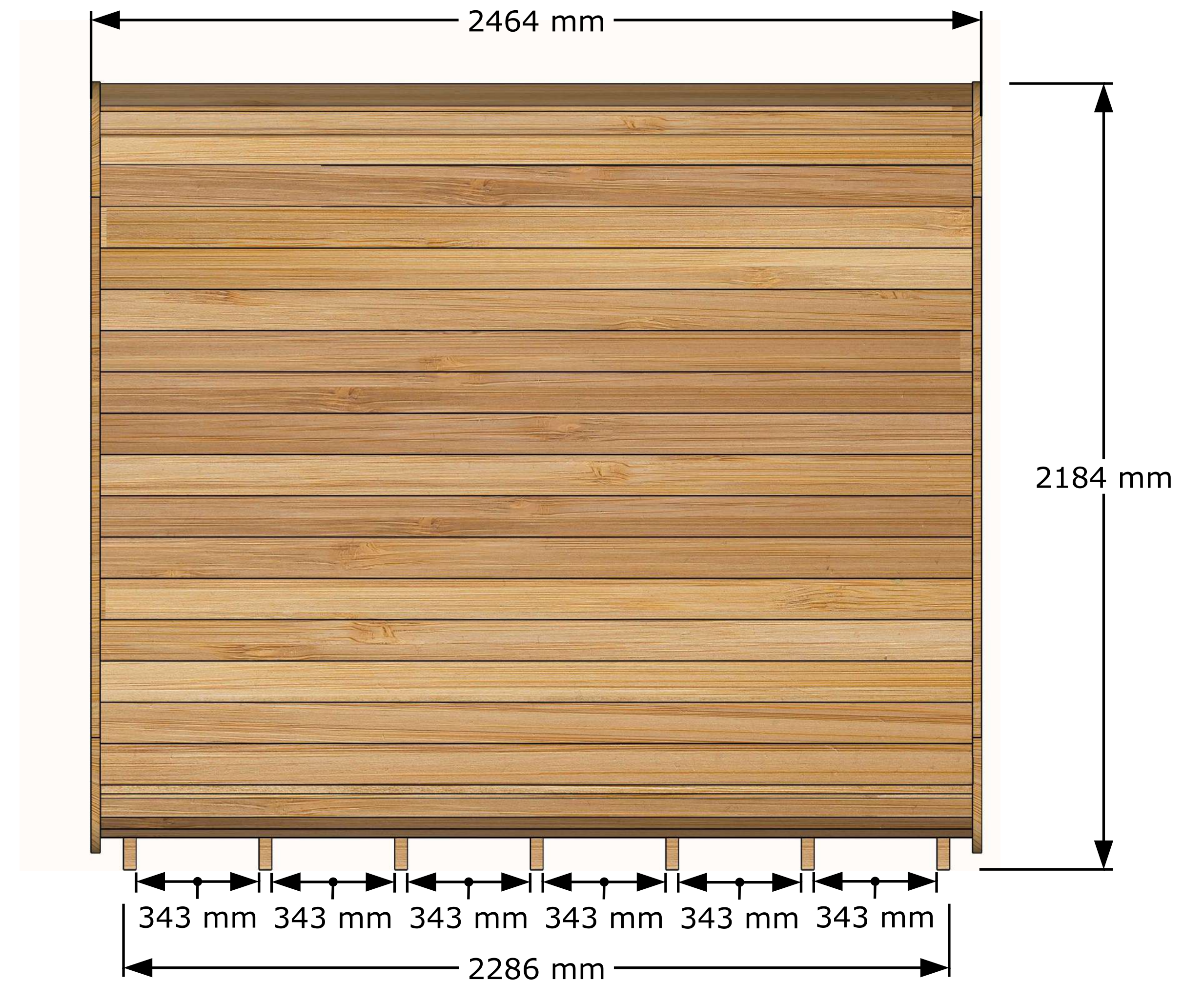
Side View
