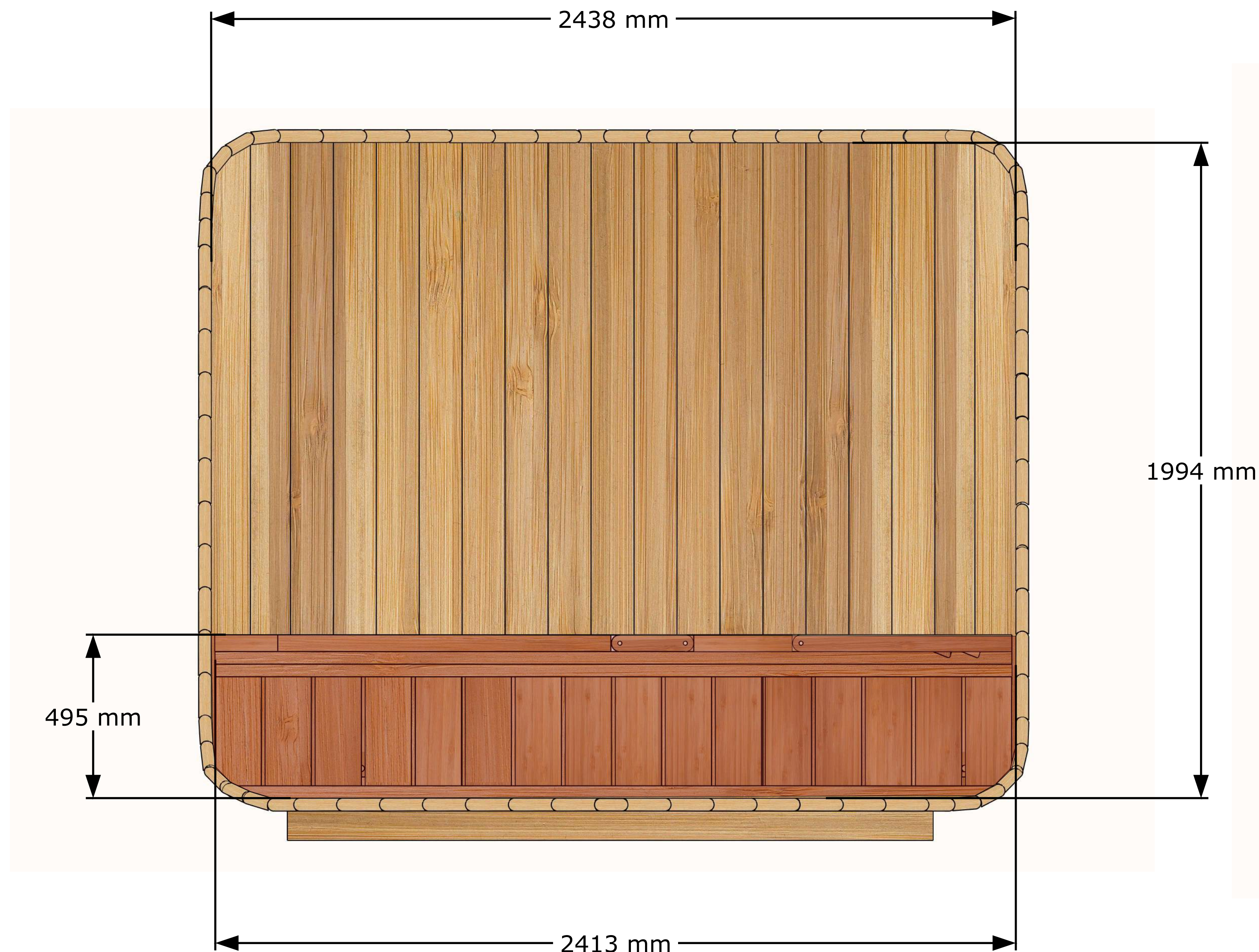
Front View
