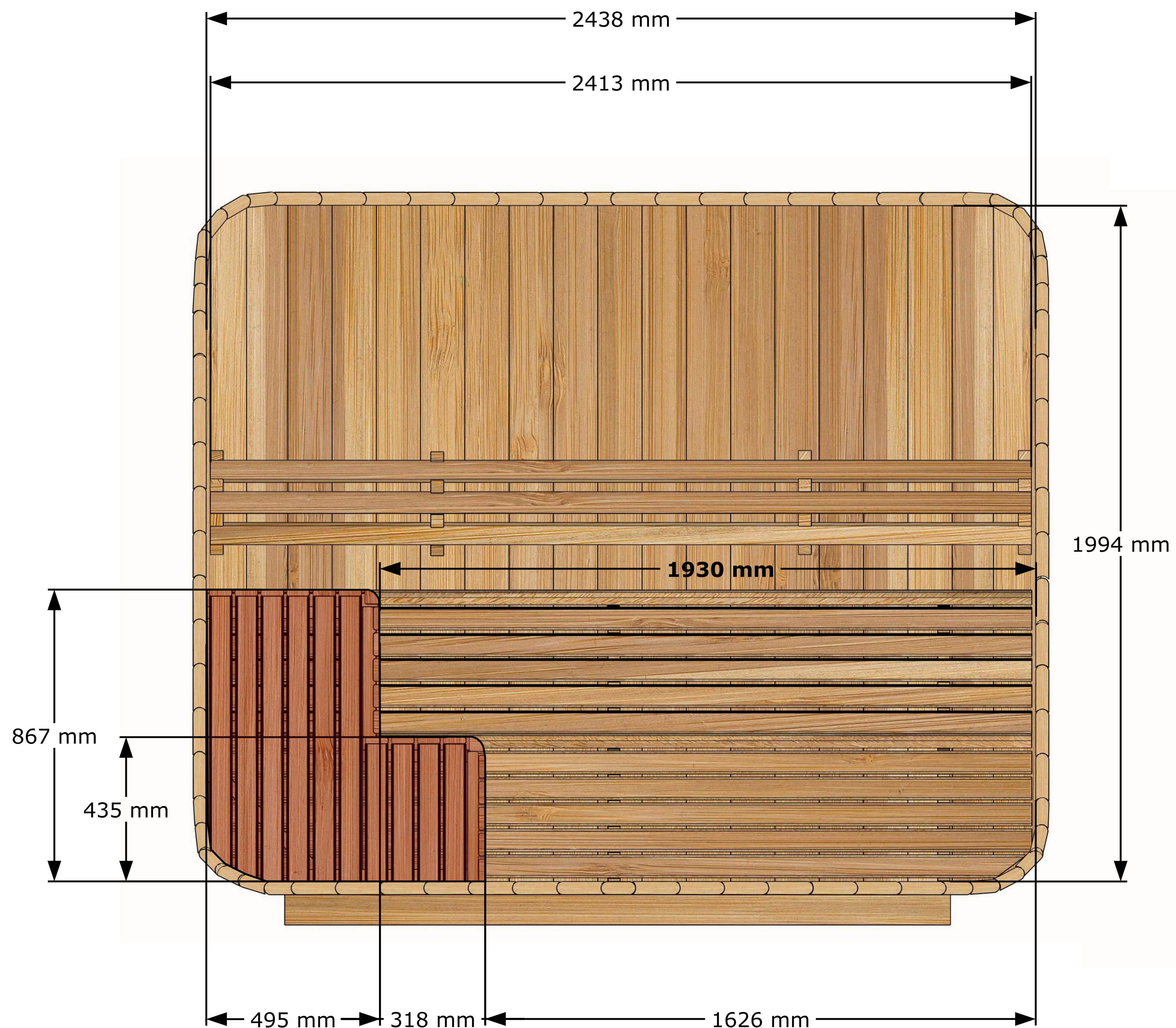
Front View
