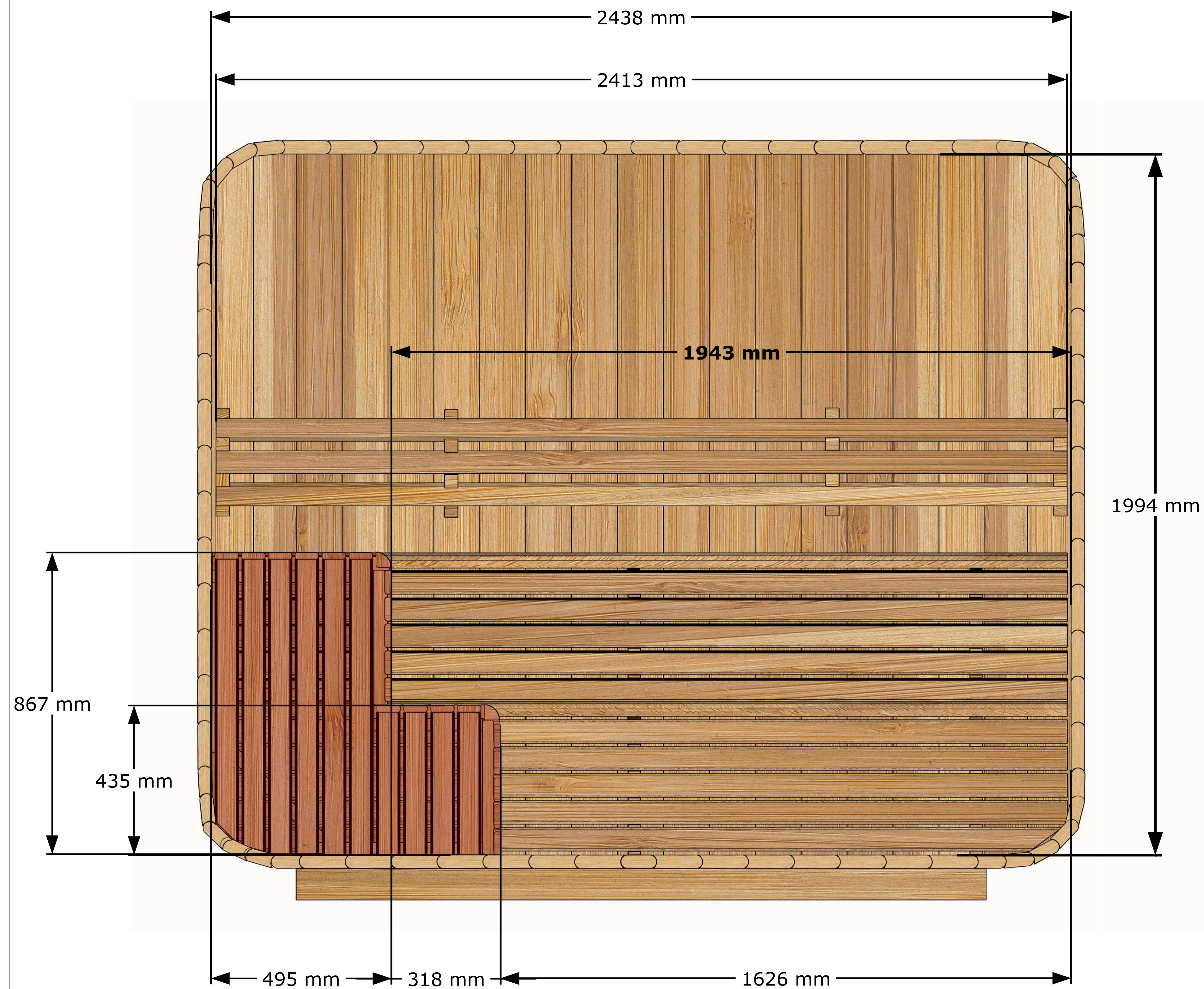
Front View
