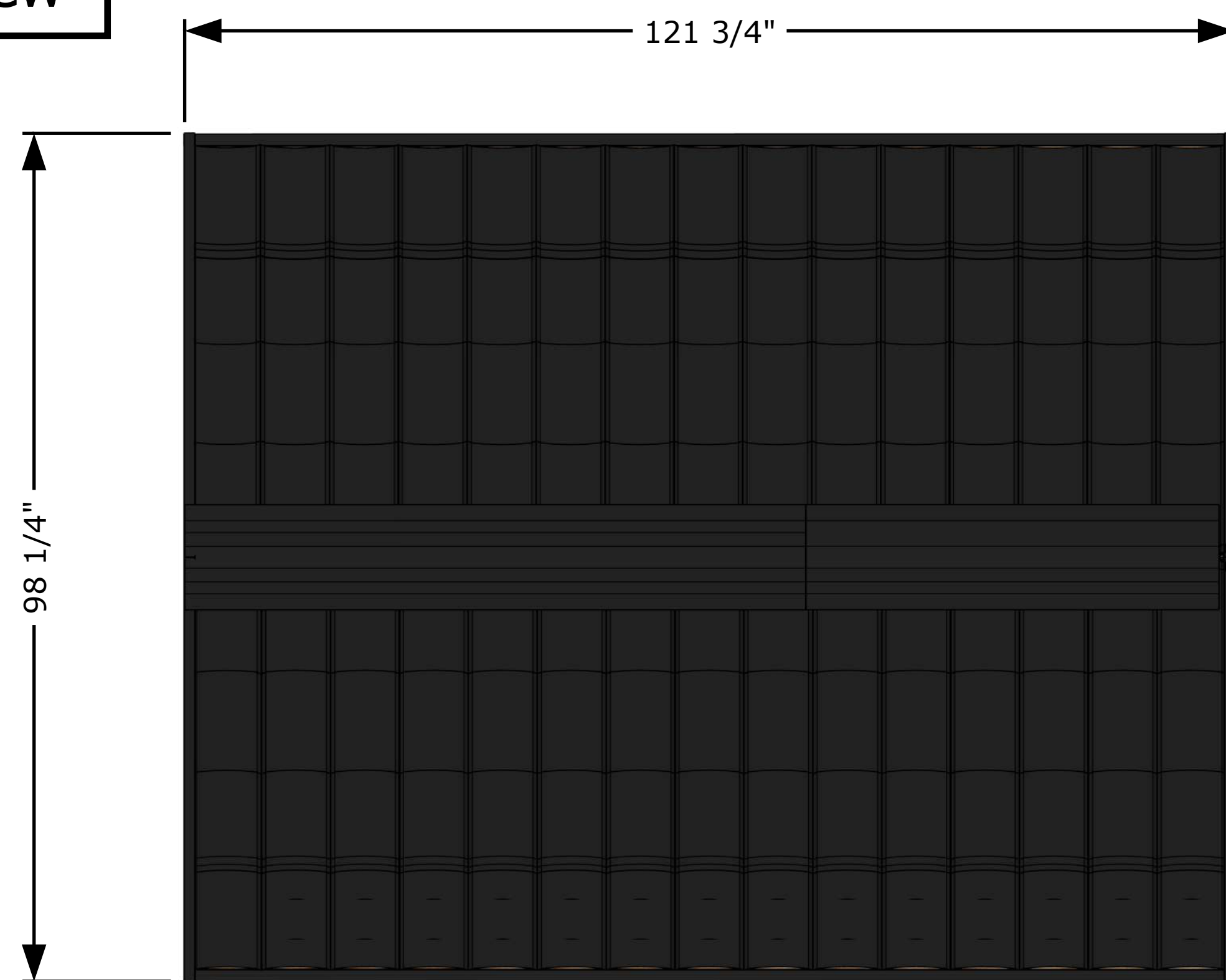
Top View
