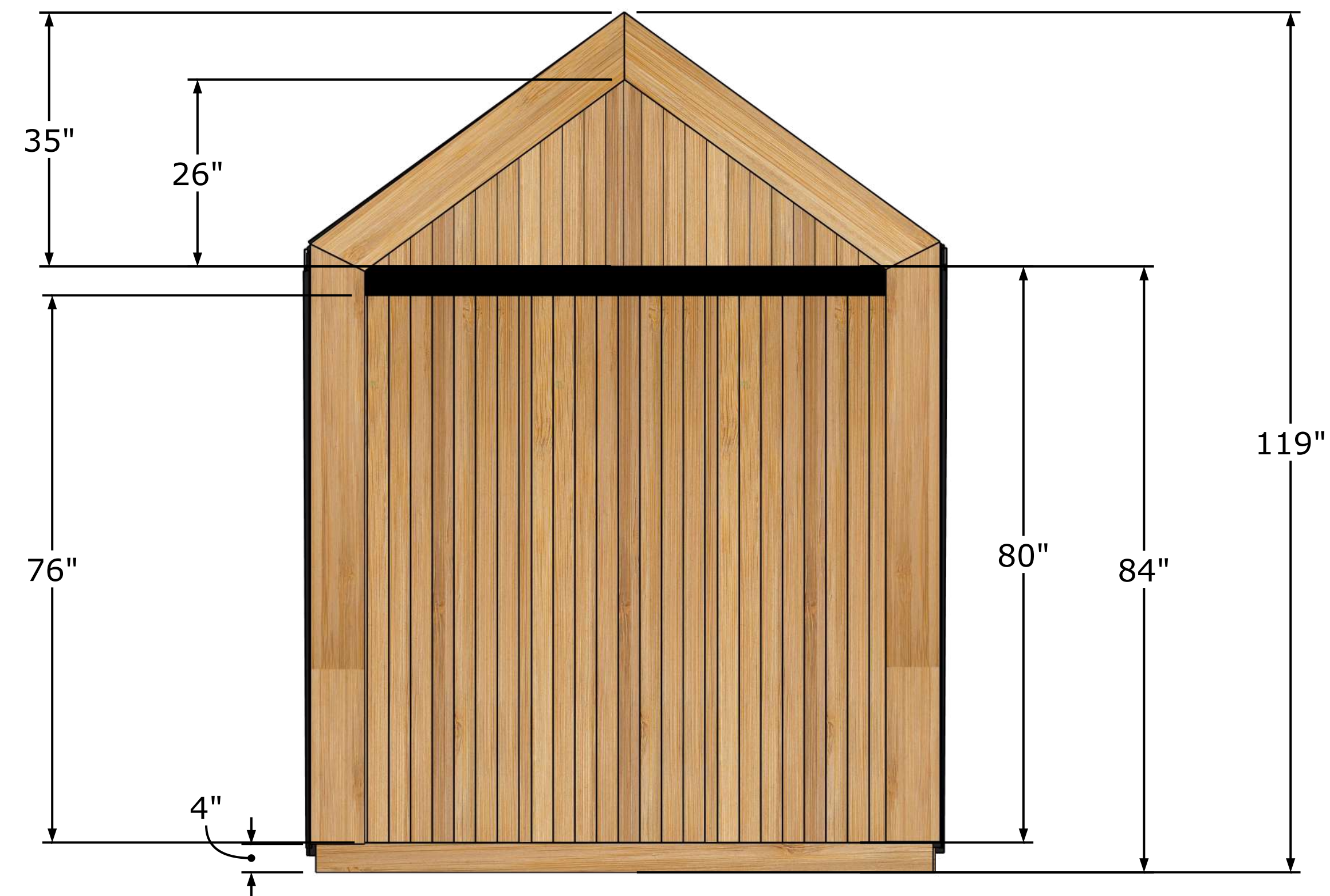
Side View
