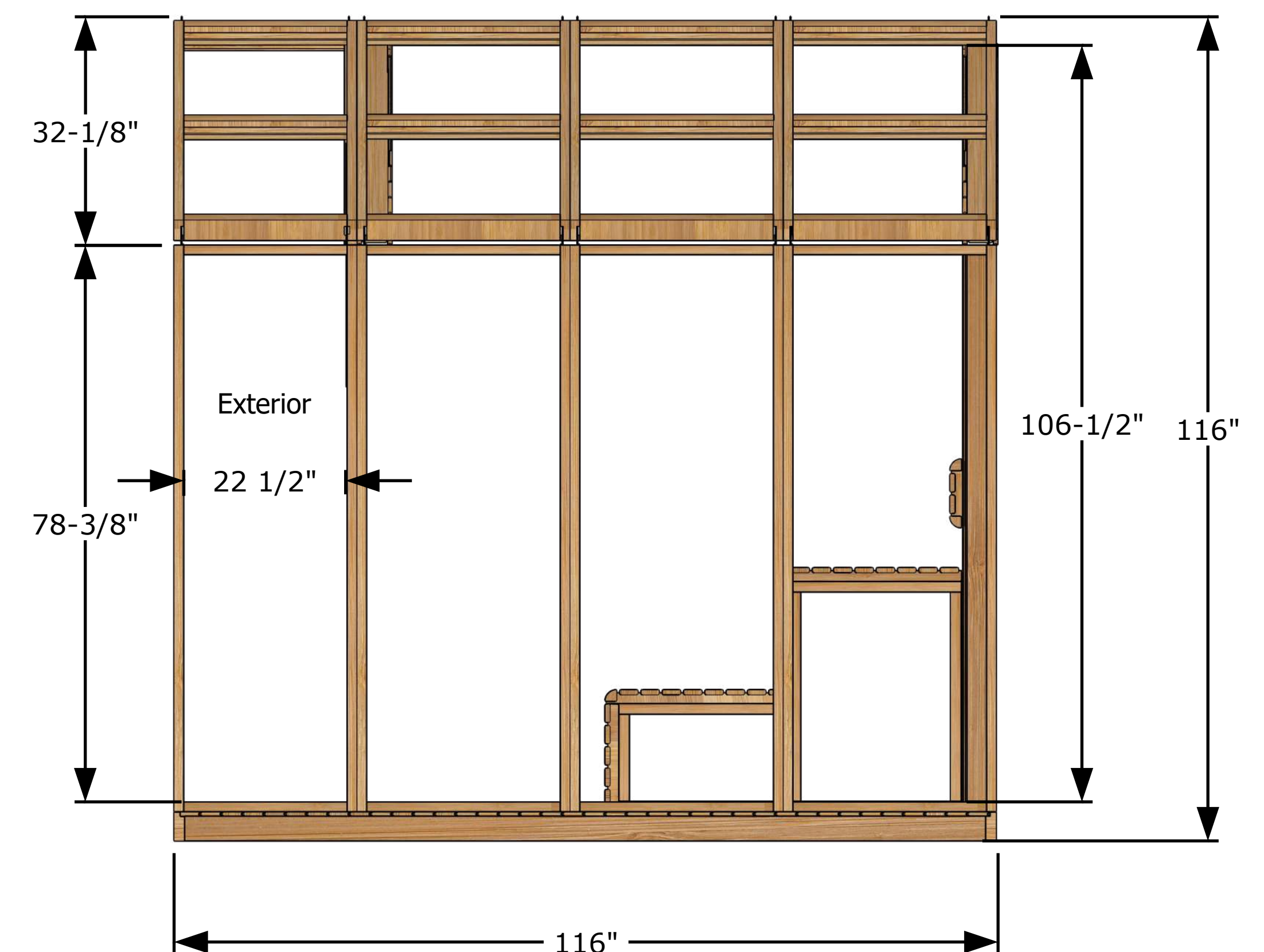
Side View
