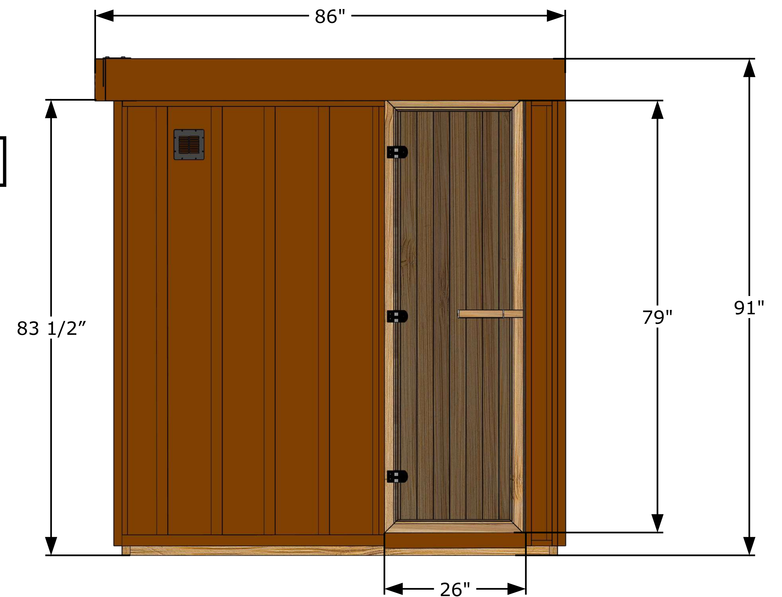
Side View
